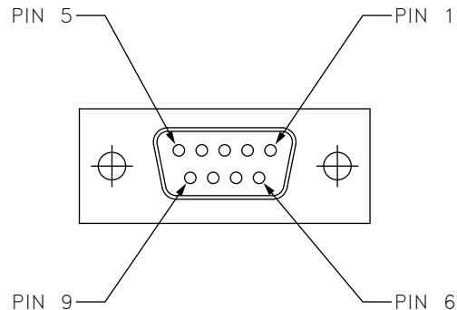
FEMALE DB-9
